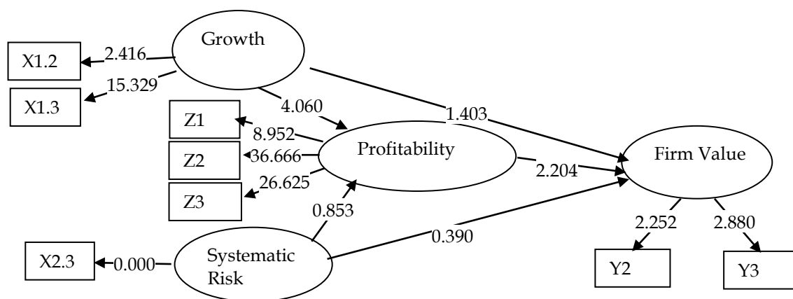
Figure 2. Output Path Coefficient/ Algorithm Model 2
