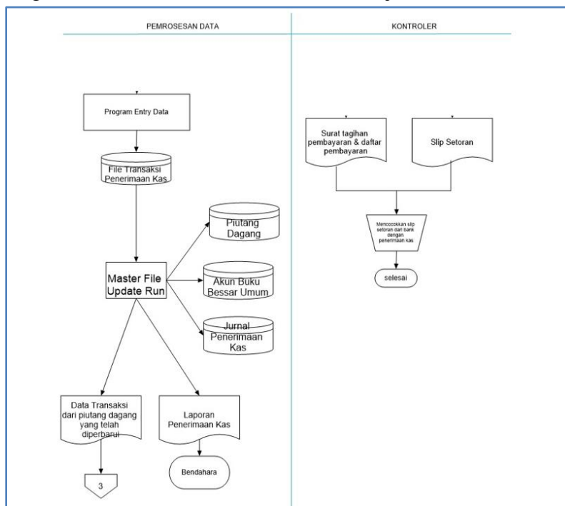
Gambar 3. Desain Flowchart
